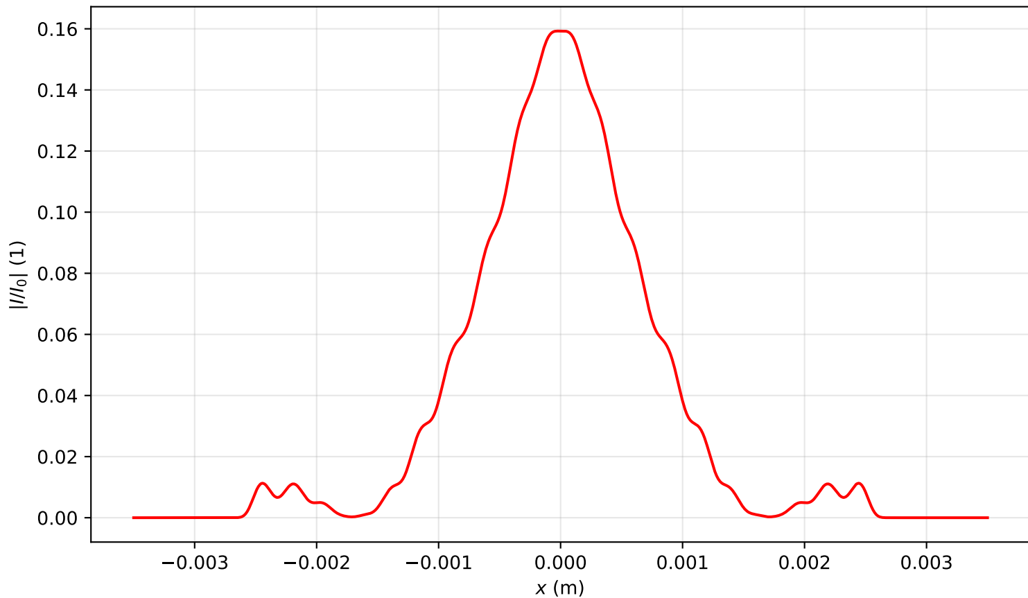
Intensity profile I(x, y = 0, z = 1.751)/I_0 , P_{in}=2.0P_{cr} , artificial time
